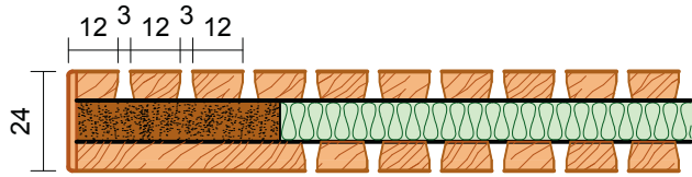
Tür-Element / Linear 12-3 / Standard
