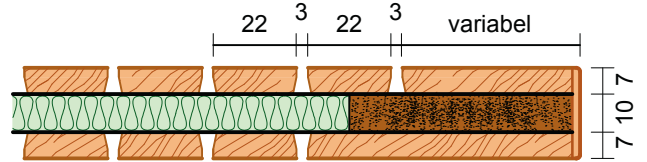
Tür-Element / Linear 22-3 / variabel
