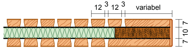
Tür-Element / Linear 12-3 / variabel
