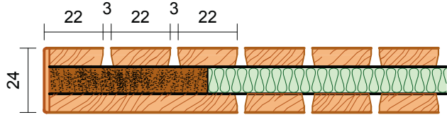
Tür-Element / Linear 22-3 / Standard
